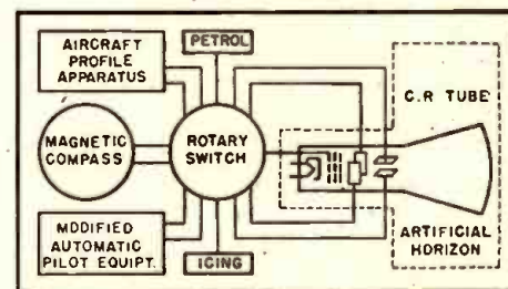
Block Diagram of British flight instrument.
